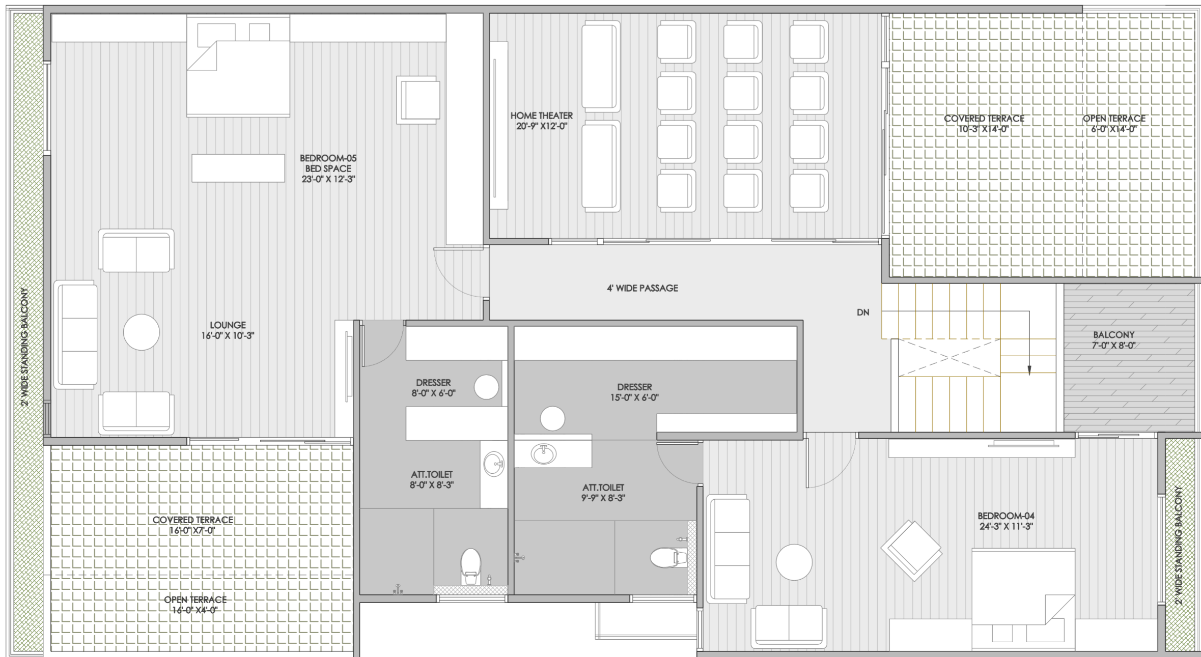
4BHK - DUPLEX UPPER FLOOR
