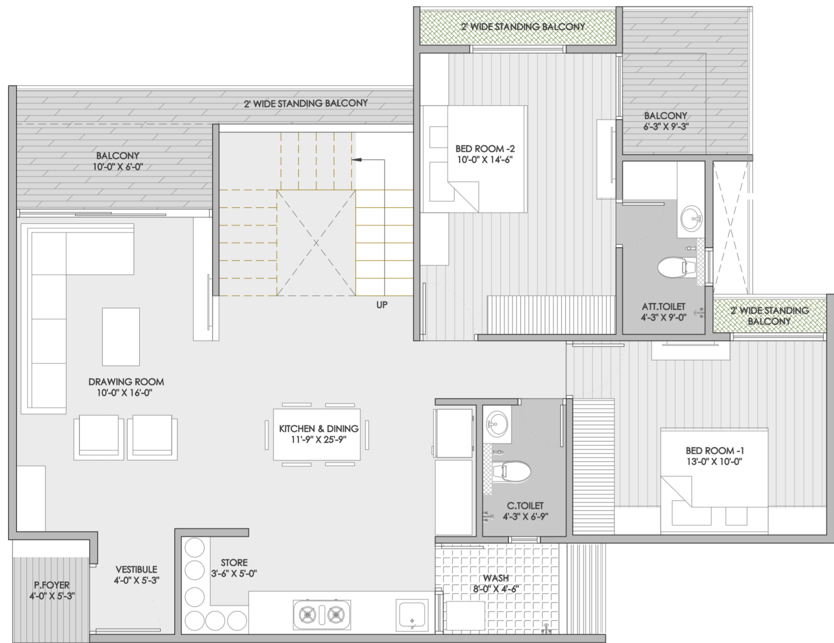
DUPLEX - LOWER FLOOR
